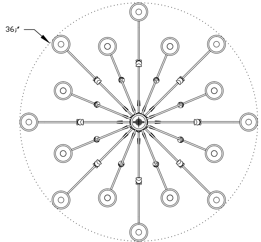
2 HANGING CHANDELIER PLAN VIEW
