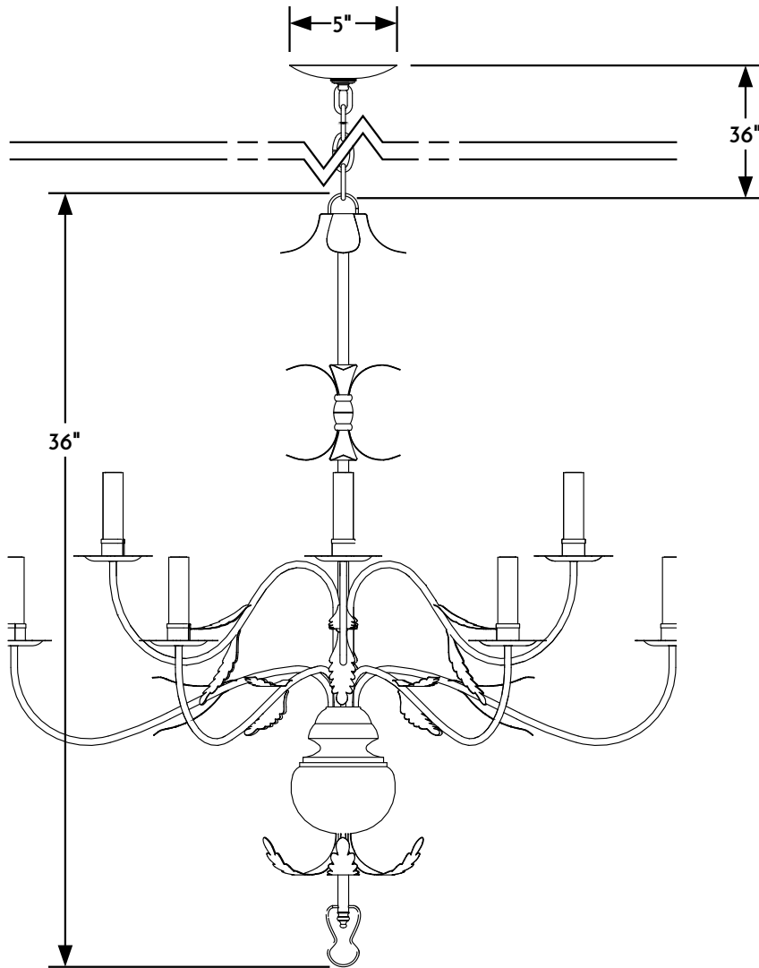
① HANGING CHANDELIER ELEVATION VIEW
