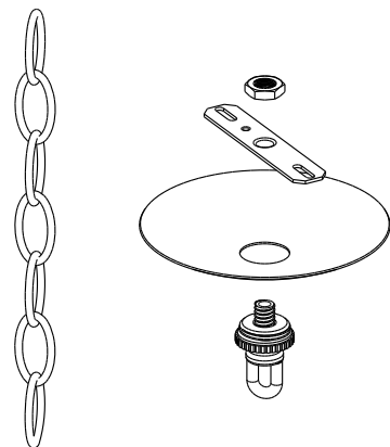
③ HANGING LANTERN CANOPY ASSEMBLY
