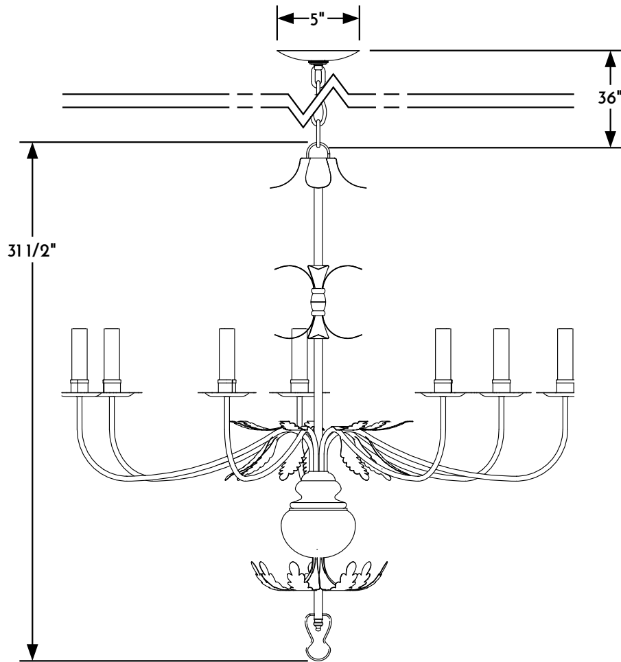
① HANGING CHANDELIER ELEVATION VIEW
