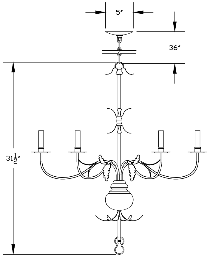
1 HANGING CHANDELIER ELEVATION VIEW
