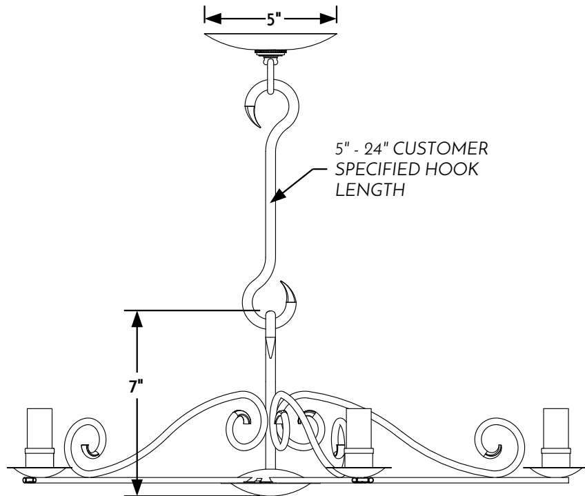
① HANGING CHANDELIER ELEVATION VIEW
